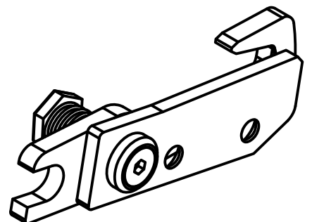
3070-00 ASSEMBLY
