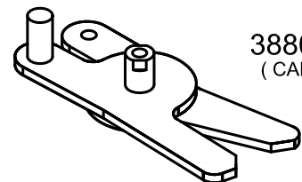
3880B-0R ASSEMBLY RH 622719000
