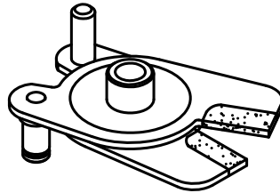
4080B-00 SCISSOR ASSEMBLY
